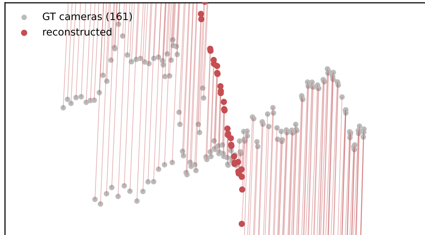
RESfM (supervised)
